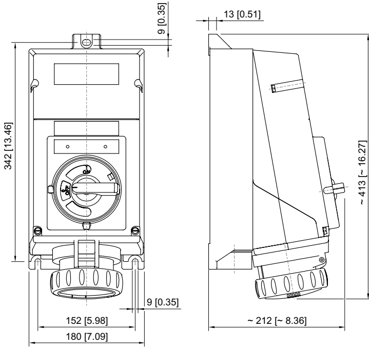
Wall-mounting receptacle
