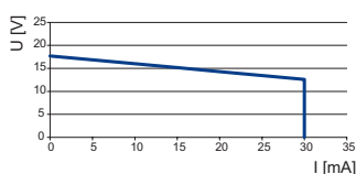
Output characteristic 9475/33-08-50
