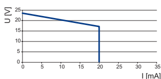
Output characteristic 9475/33-08-60
