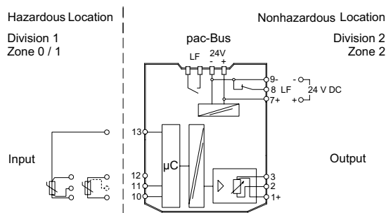
Connection Diagram 9180/10-77-11
