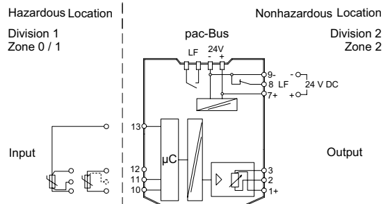
Connection Diagram 9180/10-77-11
