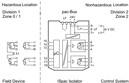
Connection diagram 9180/21-77-11
