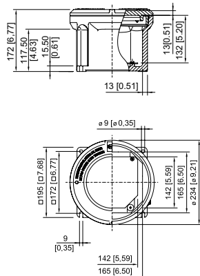
Enclosure size 3 without inspection window
