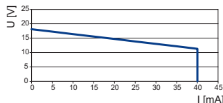
9475/32-04-12 output characteristic
