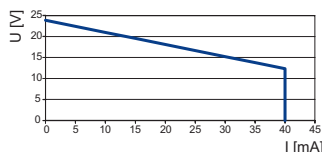
9475/32-04-22 output characteristic
