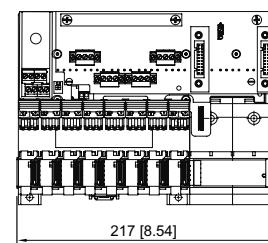
9419/04R bus-Carrier for 4 fieldbus segments
