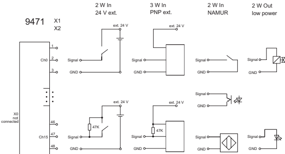
9471/35 connection diagram
