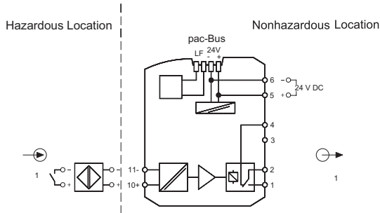
Connection diagram 9270/11-16-14
