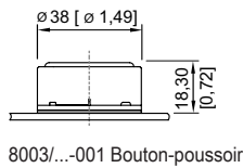
8003/...-001 Bouton-poussoir
