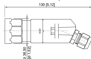
8003/...-001 Bouton-poussoir
