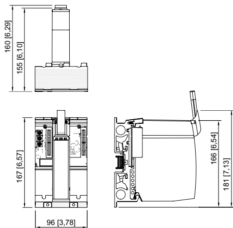
Modules Power 9445/32, 9445/35 + base 9496 (3 emplacements)
