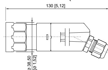
8003/...-001 Bouton-poussoir
