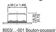
8003/...-001 Bouton-poussoir
